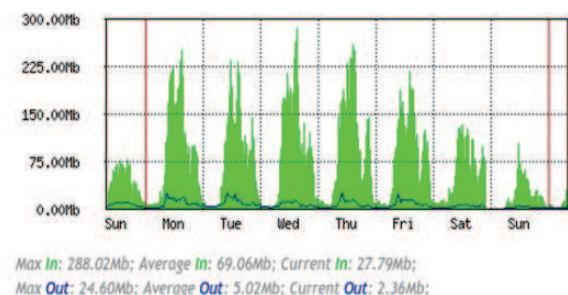
"Weekly" Graph (30 Minute Average)
